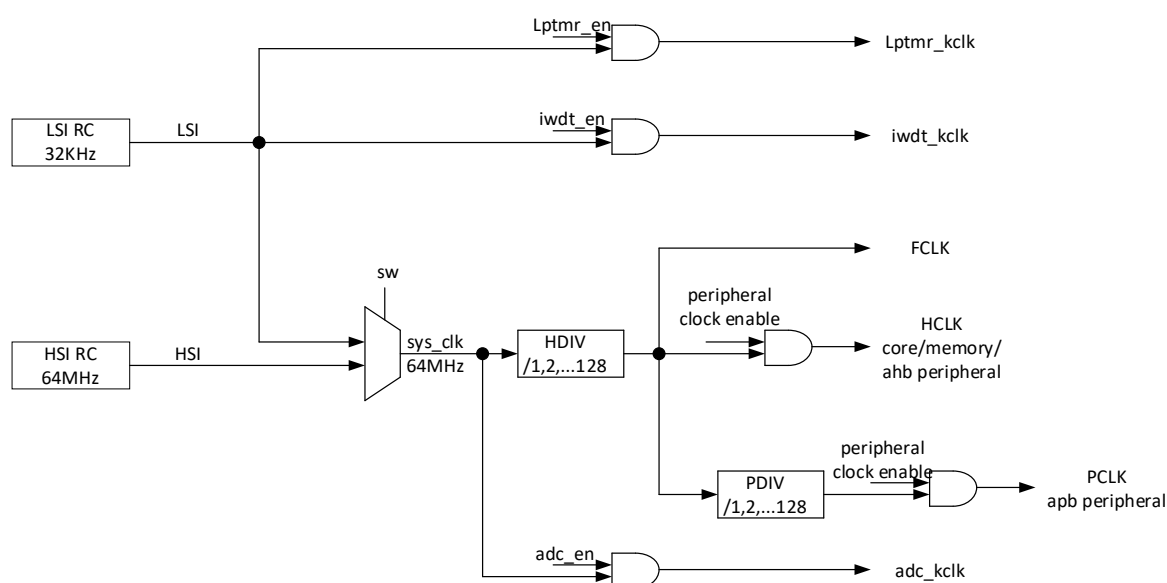
Figure 7 Clock Tree
