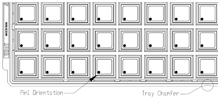
Figure 23 Tray Packaging Diagram
