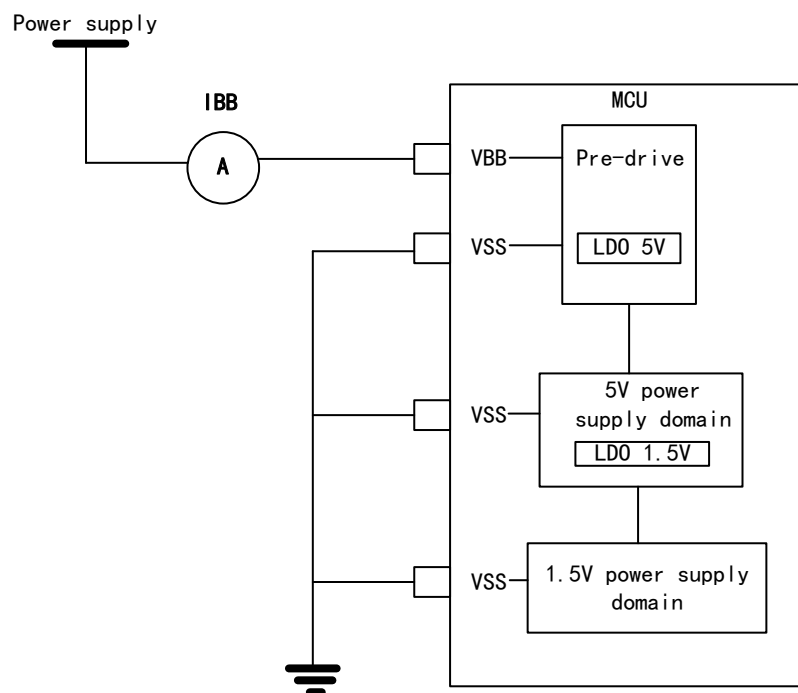
Figure 11 Power Consumption Measurement Scheme
